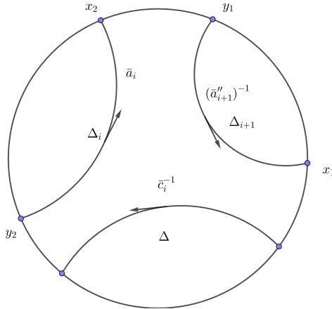
Figure 4: \Delta , \Delta_i and \Delta_{i+1} are preserved by respectively \bar{c}_i^{-1} , \bar{a}_i and (\bar{a}_{i+1}'')^{-1} . The attracting fixed point of (\bar{a}_{i+1}'')^{-1} is x_1 , and the attracting fixed point of \bar{a}_i is x_2 .
