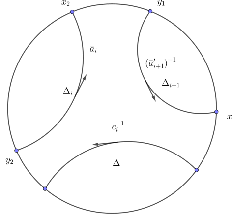
Figure 4: \Delta , \Delta_i and \Delta_{i+1} are preserved by respectively \bar{c}_i^{-1} , \bar{a}_i and (\bar{a}'_{i+1})^{-1} . The attracting fixed point of (\bar{a}'_{i+1})^{-1} is x_1 , and the attracting fixed point of \bar{a}_i is x_2 .
