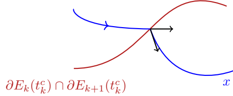
Figure 3: Geometrical illustration of a transversal boundary crossing (see Assumption (A3)).
