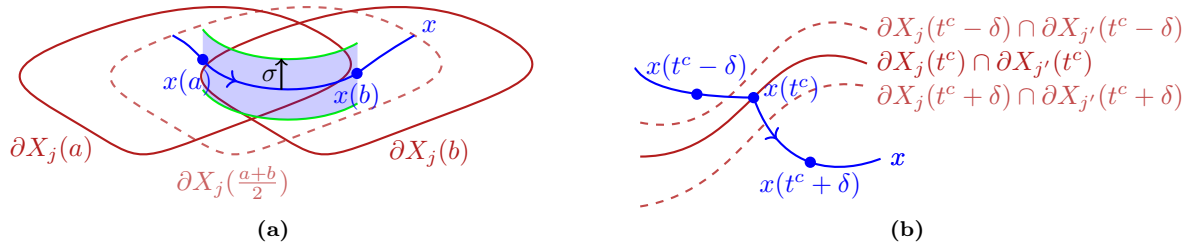
Figure 1: Illustrations of Condition (C1) on the left, and of Condition (C2) on the right.
