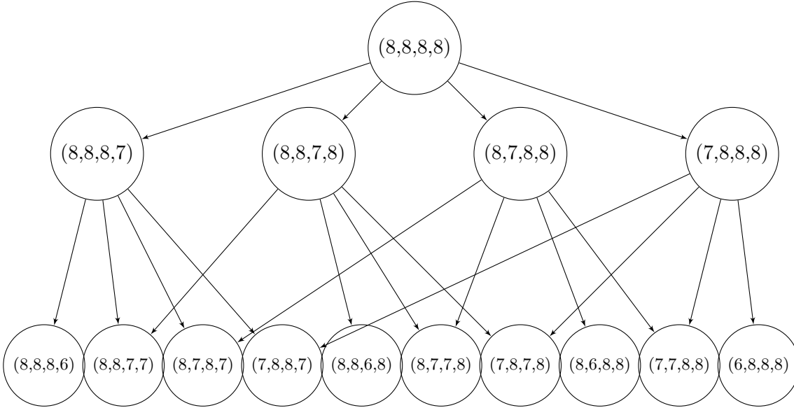
Figure 1: Subgraph for 32, 31 and 30 chessmen.
