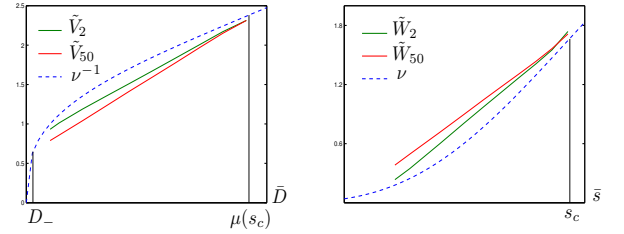
Fig. 5. Left: \tilde{V}_{T_1} , \tilde{V}_{T_2} , \nu^{-1} w.r.t. \bar{D} . Right: \tilde{W}_{T_1} , \tilde{W}_{T_2} , \nu w.r.t. \bar{s} (for Hill kinetics with T_1 = 2 , T_2 = 50 , s_{in} = 6 , m = 5 , K = 3 , n = 3 , D_+ = 4.5 , D_- = 0.05 )
