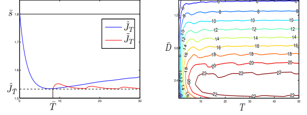
Fig. 4. Left: costs \hat{J}_T , \tilde{J}_T for the Hill law with s_{in} = 6 , m = 5 , K = 3 , n = 3 , D_+ = 4.5 , D_- = 0.05 , \bar{s} = 1.8 , where \bar{T} \simeq 8.21 . Right: Iso-values of \tilde{G}_1 (for the Hill function) in %.
