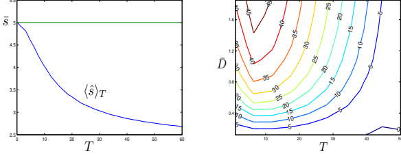
Fig. 2. Left: optimal cost w.r.t. T for the Contois law with s_{in} = 8 , m = 2 , K = 5 , D_+ = 1.95 , D_- = 0.02 , \bar{D} = 0.5 . Right: Iso-values of G_1 (for the Contois function) in %.
