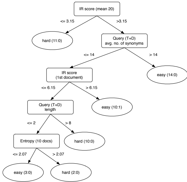
Figure 3: Decision tree related to ok8amxc, reduced feature set
