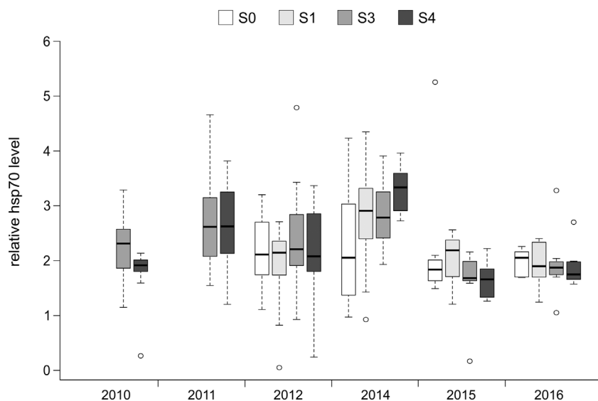
Fig. 14. Relative Hsp70 levels in kidney of feral chub, depending on sampling site and year. Comparison of the situations prior (2010–2012) and subsequent (2014–2016) to the WWTP upgrade. Bold lines within boxes display the median values, boxes the 25% to 75% quantiles, whiskers the minimum and maximum values, circles potential outliers. S0 = Schussen River, upstream of SOB and WWTP Langwiese. S1 = Schussen River, downstream of SOB and upstream of WWTP Langwiese. S3 = Schussen River, downstream of WWTP Langwiese. S4 = Argen River, reference river. Site 0: n = 0 (2010, 2011), n = 24 (2012), n = 20 (2014), n = 9 (2015), n = 5 (2016). site 1: n = 0 (2010, 2011), n = 22 (2012), n = 19 (2014), n = 10 (2015); n = 9 (2016). site 3: n = 20 (2010), n = 28 (2011), n = 24 (2012), n = 20 (2014), n = 10 (2015), n = 9 (2016). site 4: n = 16 (2010), n = 18 (2011), n = 20 (2012), n = 6 (2014), n = 5 (2015), n = 8 (2016). 2010–2012 prior to the WWTP upgrade, 2014–2016 after the upgrade. A significant influence of the sampling year was found (ANOVA, F(5, 11) = 12.1 , p < 0.0001 ).
