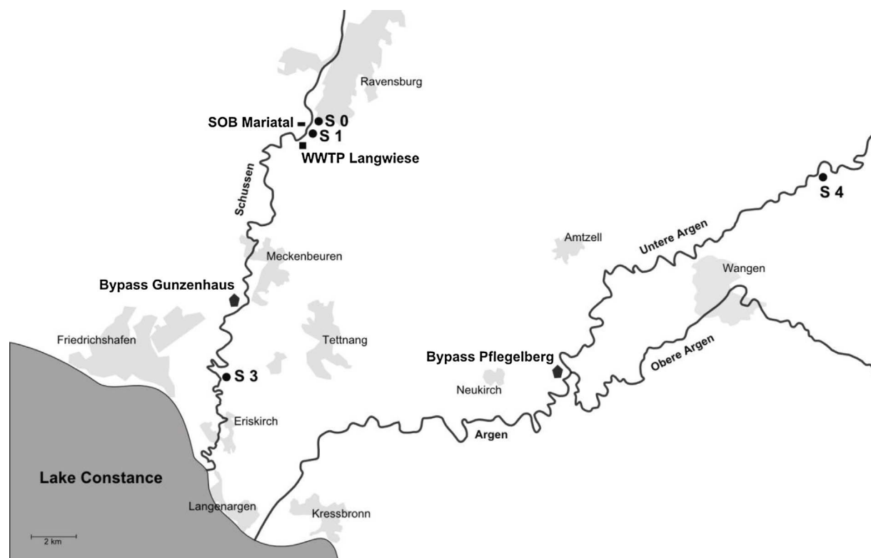
Fig. 1. Location of the WWTP Langwiese, the bypass systems, and the field sampling sites. WWTP: wastewater treatment plant. SOB: stormwater overflow basin. Bypass Gunzenhaus: bypass station at the Schussen River. Bypass Pfflegelberg: bypass station at the Argen River. Field sampling sites: S0: Schussen River, Weissenau, upstream of SOB and WWTP Langwiese. S1: Schussen River, Weissenau, downstream of SOB and upstream of WWTP Langwiese. S3: Schussen River, Oberbaumgarten, downstream of WWTP Langwiese. S4: Argen River, Oberau, reference river.
